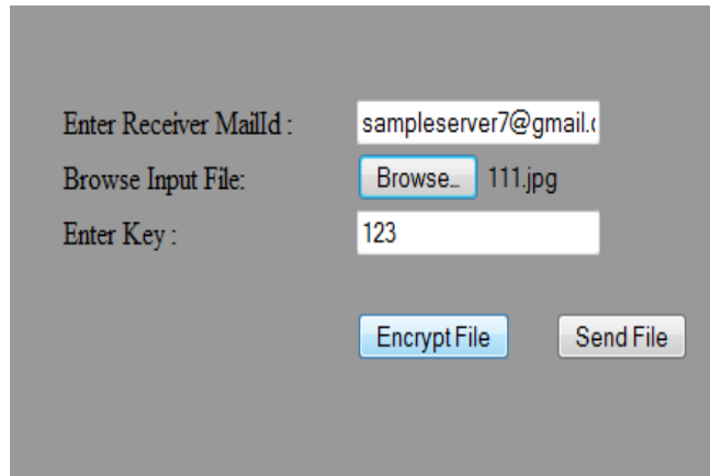
Figure 8 Image encryption
