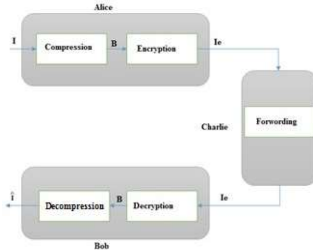
Figure 1. Traditional Compression-then-Encryption (CTE) system.
