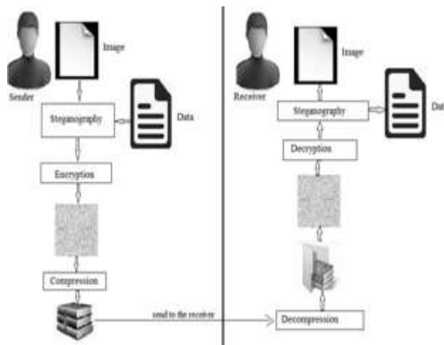
Figure 4 System Architecture
